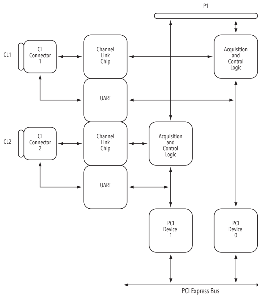
Figure 1-2 NEO-PCE-CLD Block Diagram
