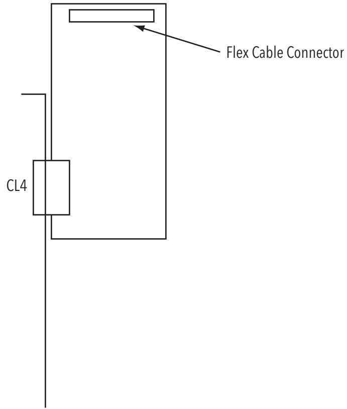
Figure 13-5 NEO-PCE-CLQ CL4 Connector
