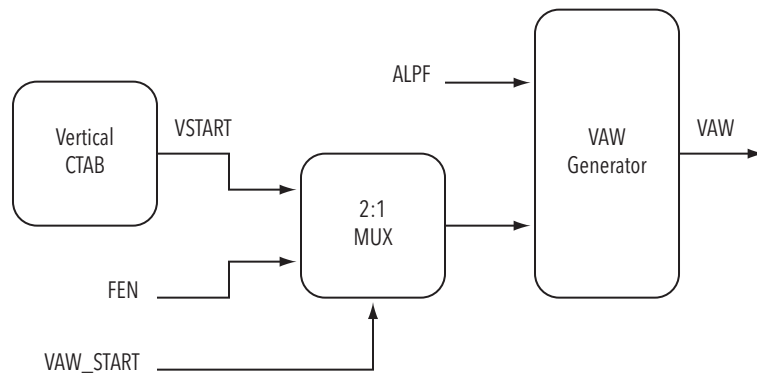
Figure 2-5 Generation of the Vertical Active Window, VAW
