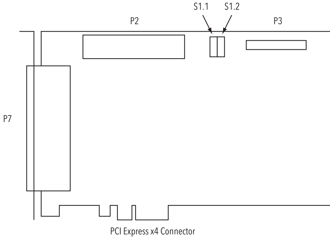
Figure 13-6 NEO-PCE-DIF Layout
