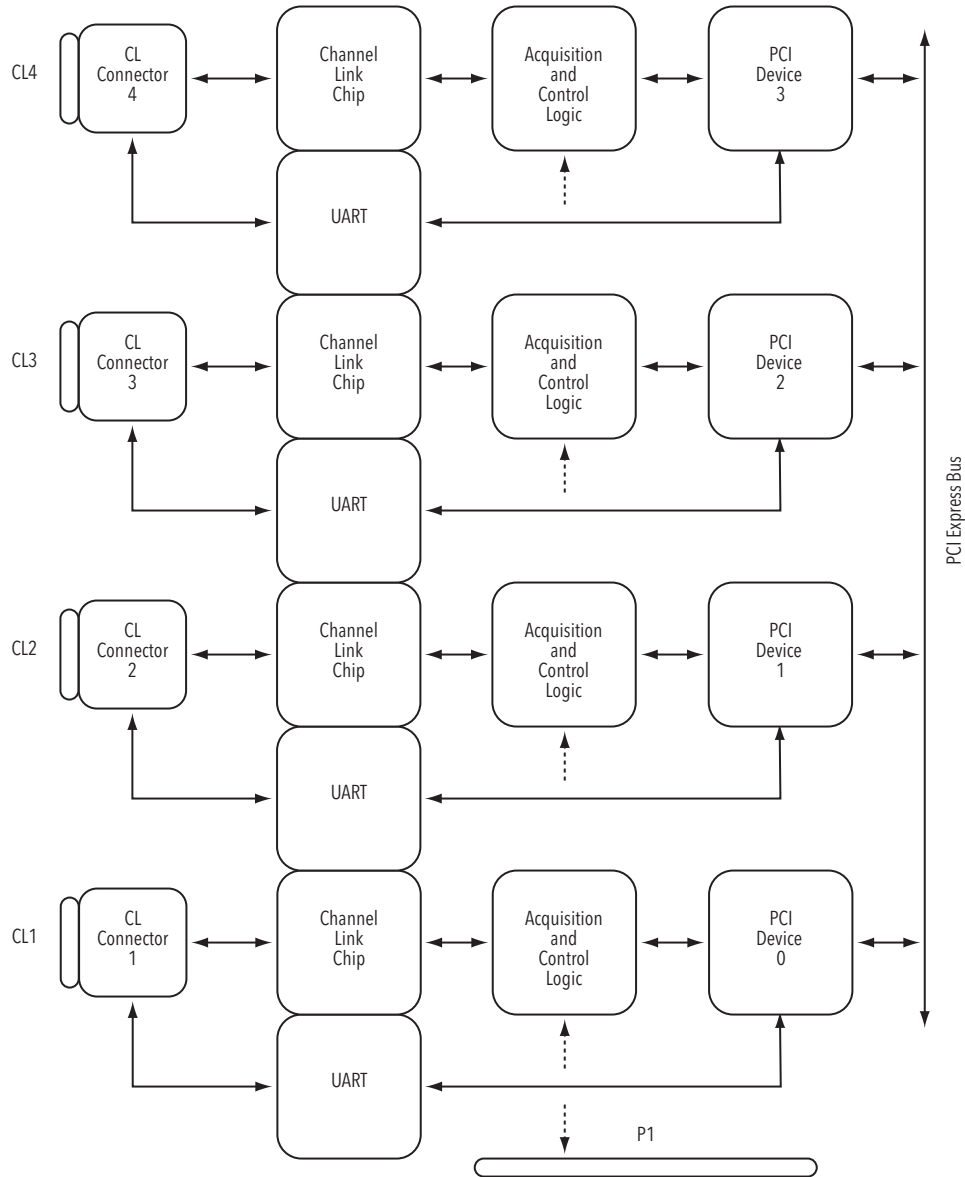
Figure 1-3 NEO-PCE-CLQ Block Diagram
