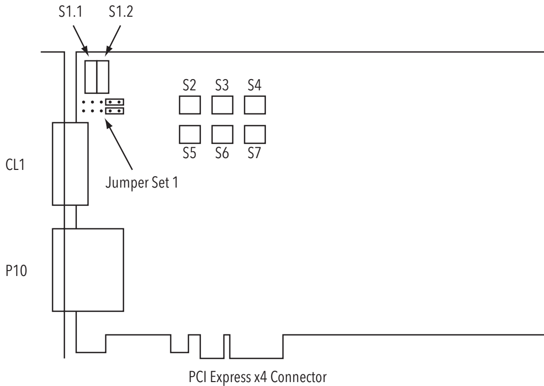
Figure 13-2 NEO-PCE-CLB Revision 2 Layout
