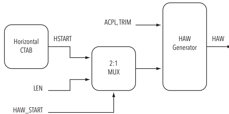
Figure 2-4 Generation of the Horizontal Active Window, HAW
