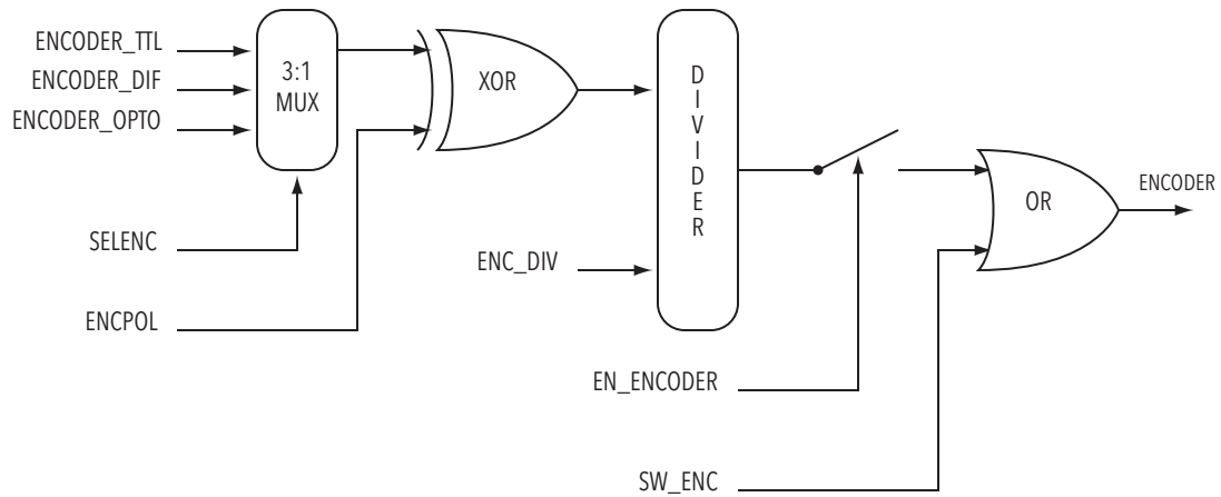
Figure 2-14 Encoder Circuit
