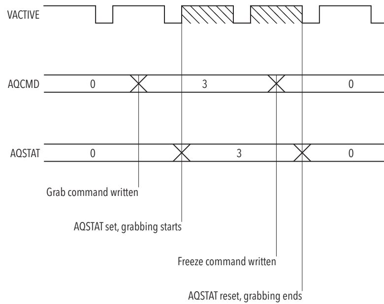
Figure 2-9 Grab Command Timing
