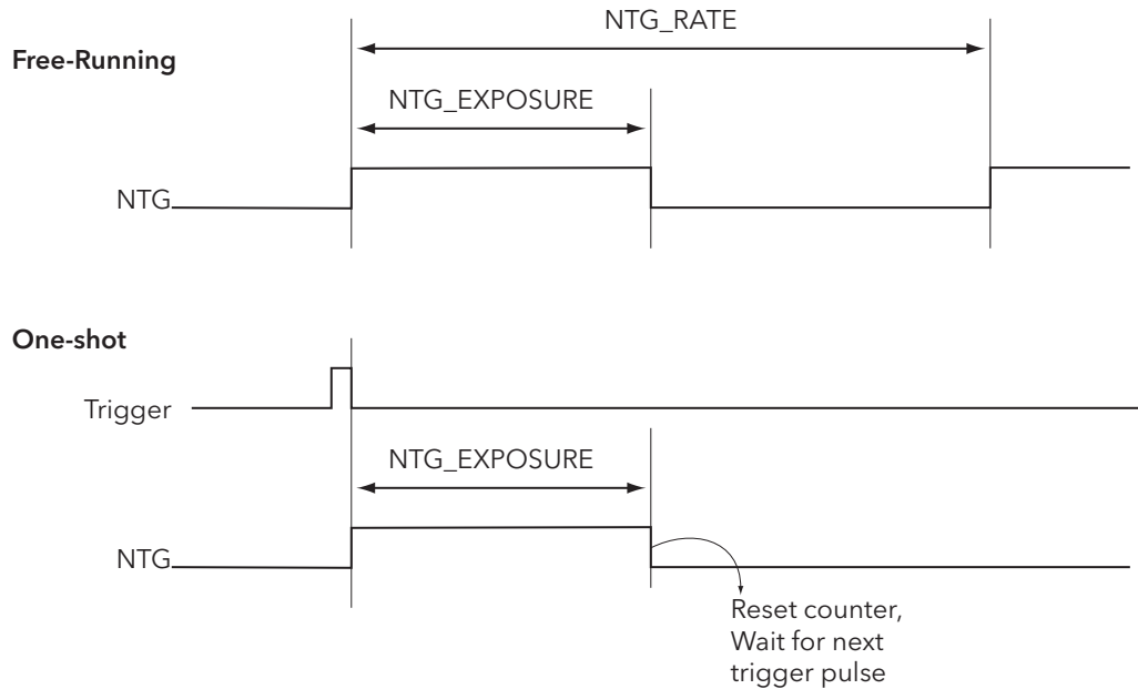
Figure 3-1 NTG Timing
