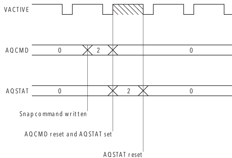
Figure 2-8 Snap Command Timing
