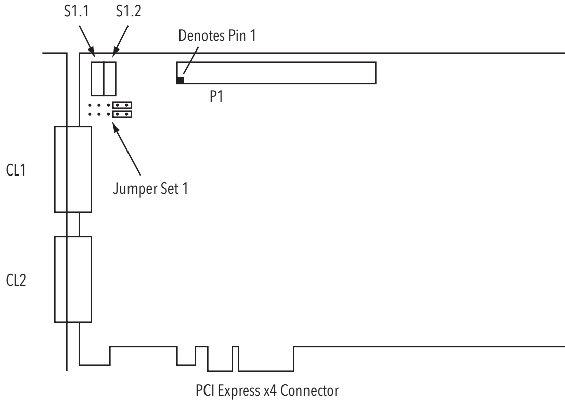
Figure 13-3 The NEO-PCE-CLD Layout
