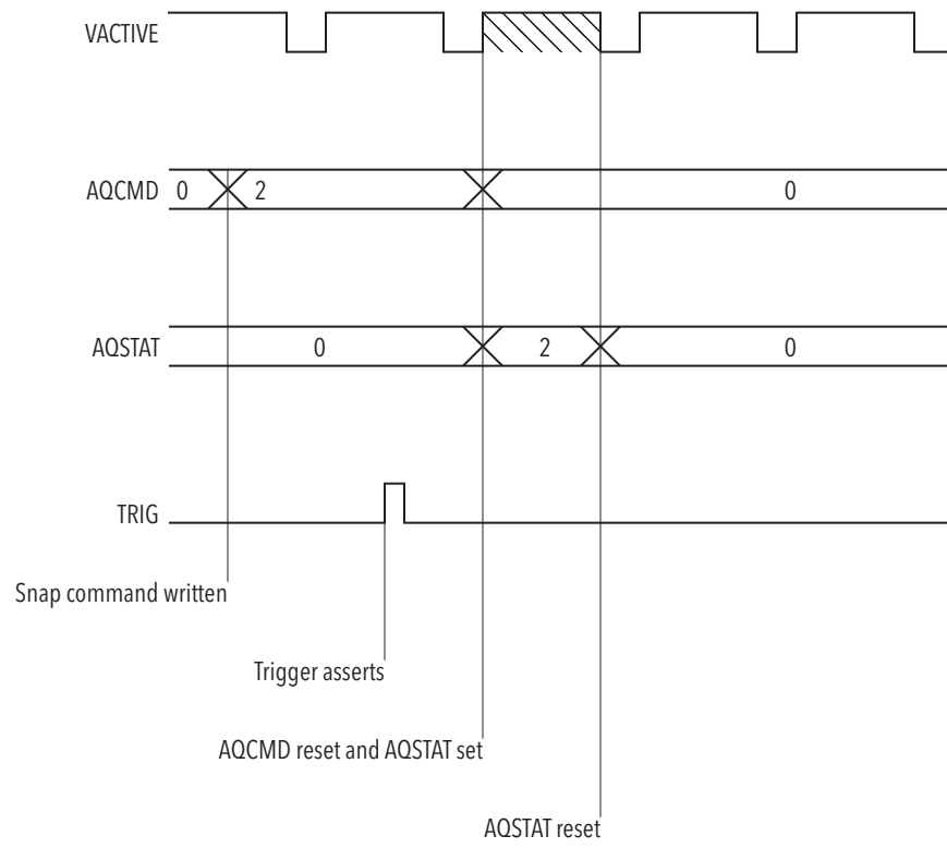
Figure 2-11 Snap Command Timing with ACQ_CON = 2
