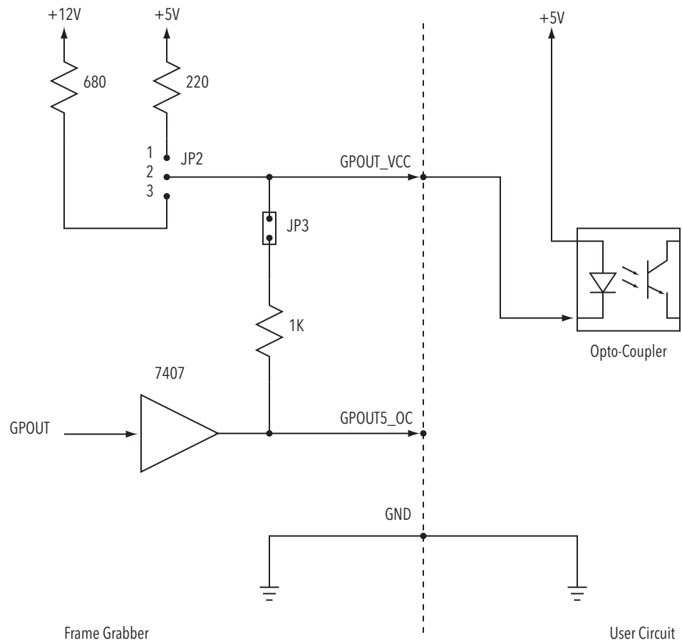
Figure 11-3 GPOUT Driving Opto-Coupled Circuit (in Default Configuration)
