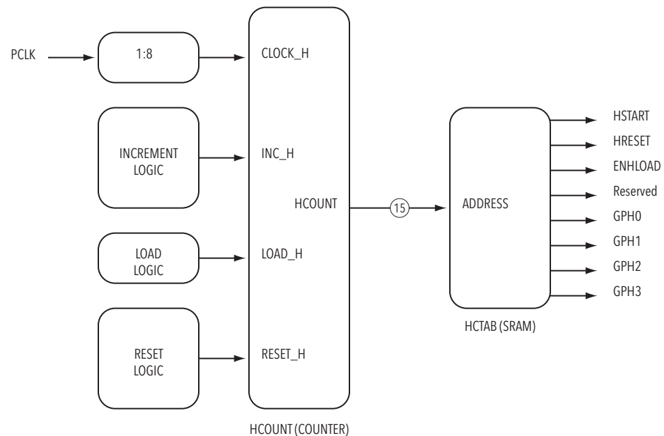
Figure 2-7 Horizontal Control
