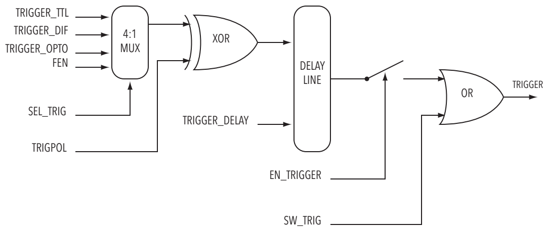
Figure 2-13 Trigger Circuit
