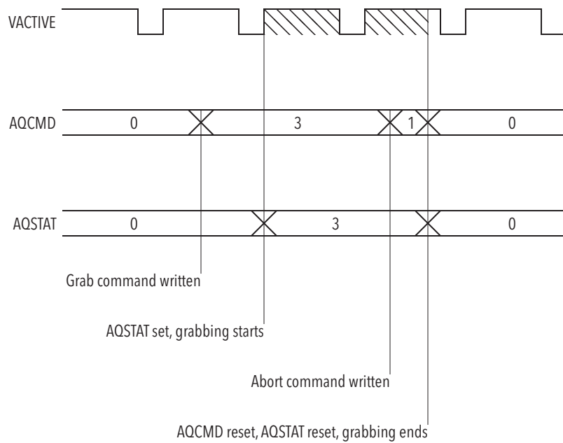
Figure 2-10 Abort Command Timing
